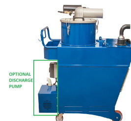
CS-300L (COOLANT/OIL) Side View
