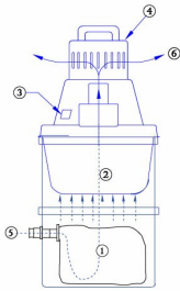
EMI-1000 Air Flow Schematic for Stainless Steel Model
